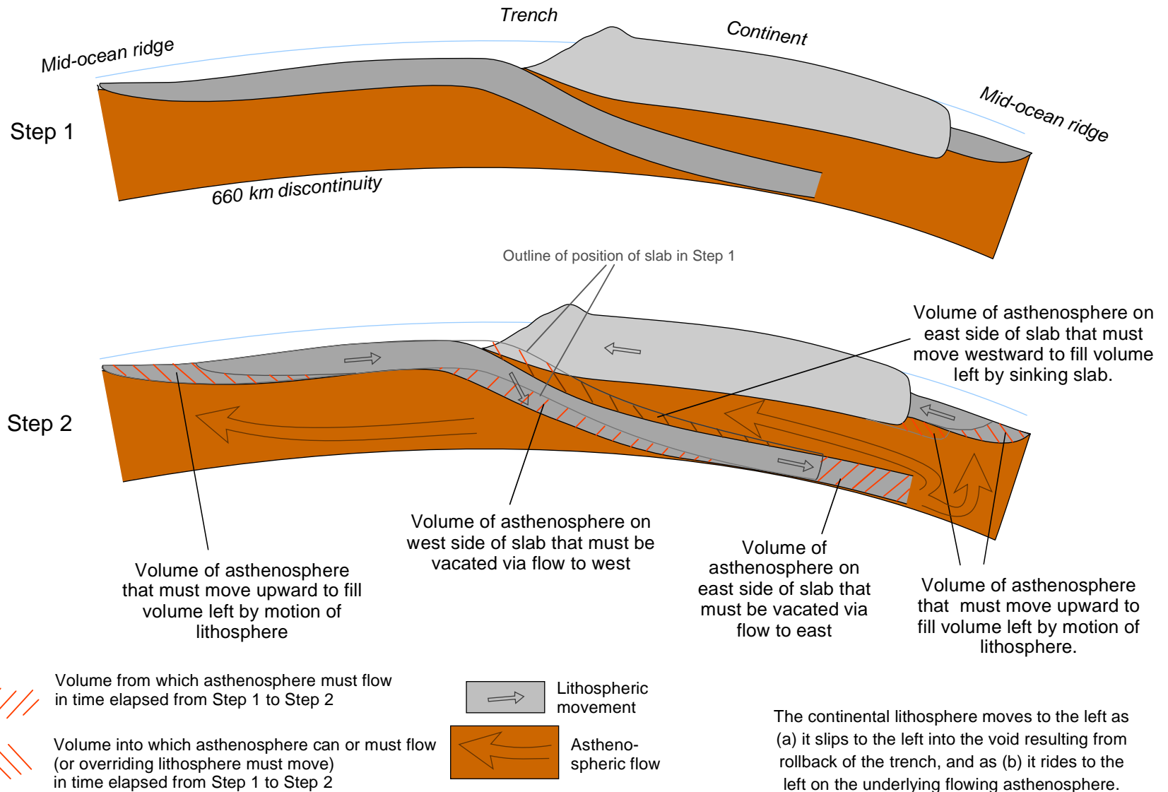
A model of rollback and mantle flow (but not mantle convection)
